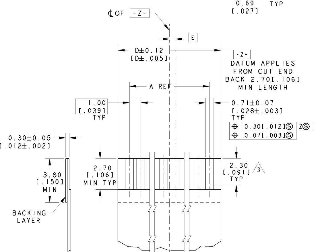
RECOMMENDED FPC LAYOUT SCALE 8:1
